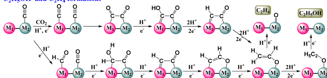
Scheme 1 Plausible mechanism for the formation of \text{C}_1 and \text{C}_2 products by the \text{eCO}_2\text{RR} using DACs.
