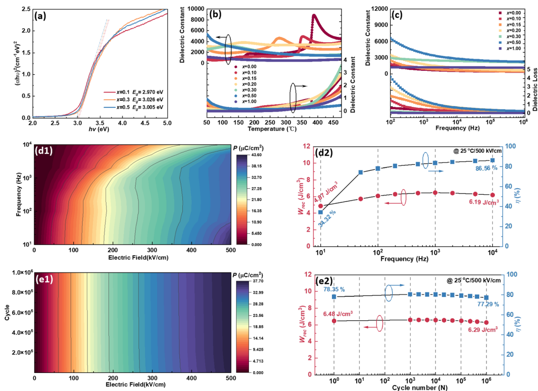
Fig. 6 (a) The fitting results of Fig. S6 † according to eqn (15) to obtain the E_g of (1-x) KNN- x BCZT with x = 0.1, 0.3 , and 0.5 ; (b) the \varepsilon-T curves with \tan \delta-T curves of the (1-x) KNN- x BCZT ceramics from 50^\circ\text{C} to 475^\circ\text{C} at 1000\text{ Hz} ; (c) the \varepsilon-f curves with the \tan \delta-f curves of the (1-x) KNN- x BCZT ceramics from 10^2 to 10^6\text{ Hz} at room temperature; (d1) the mapping to show the variation between polarization and both the applied frequency and the electric field; (d2) the variation between both W_{\text{rec}} and \eta and frequency; (e1) the mapping to show the variation between polarization and both the cycling number and the electric field; (e2) the variation between both W_{\text{rec}} and \eta and the cycling number.
