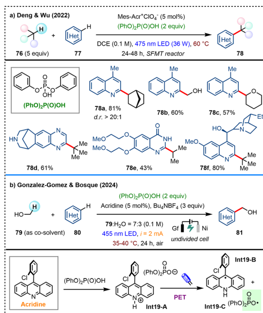
Scheme 19 Phosphate radical enabled visible-light induced CDC reaction of heteroarenes with alkanes/alcohols.
