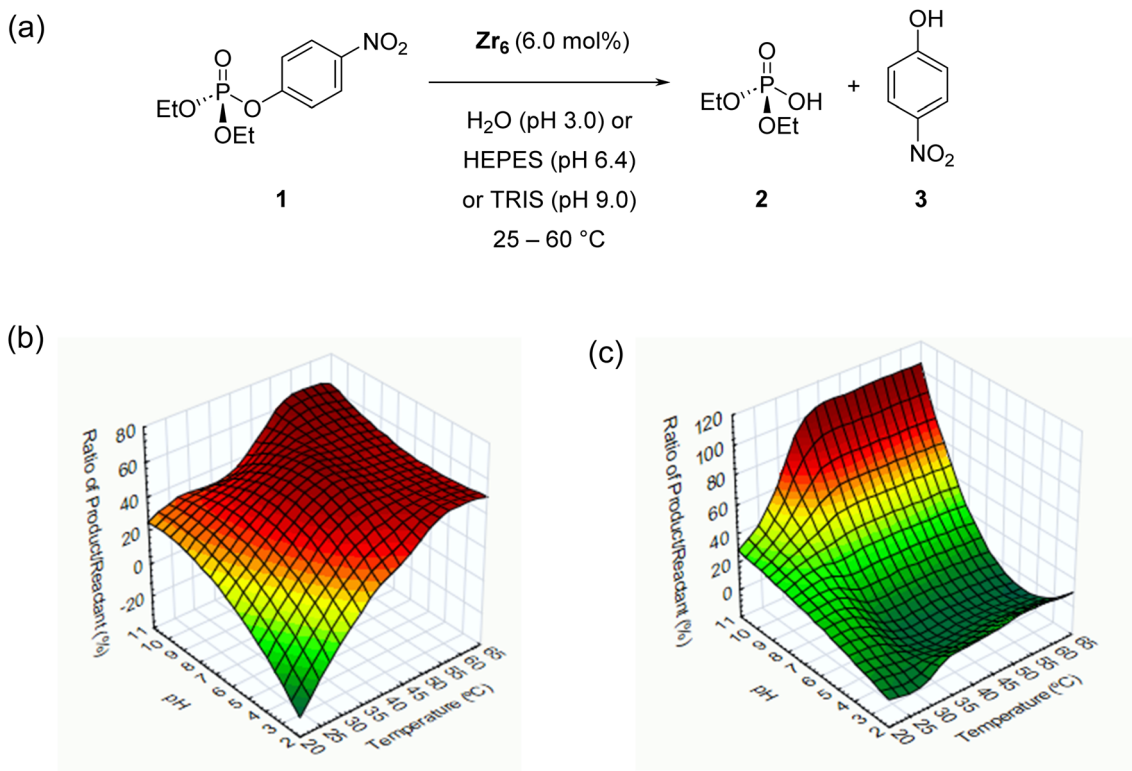
Scheme 1 (a) Reaction conditions studied for the hydrolysis of paraxon ( 1 ) with the Zr_6 cluster. (b) Results of initial screening using Zr_6 as the catalyst. (c) Results of spontaneous hydrolysis of ( 1 ) under the same screening conditions. Results are presented as the percentage ratio of product/reactant by integration of peaks in ^1H NMR data. Green color represents lower yields, while red color represents higher yields.
