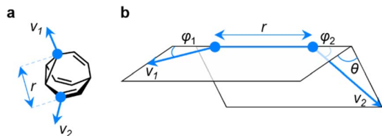
Fig. 5 (a) The vectors v_1 and v_2 for two substituent attachment points on a BV (shown for (\alpha S)-\gamma,\delta' - \text{Me}_2\text{BV} ) which are defined by (b) the geometric parameters r , \phi_1 , \phi_2 , and \theta .
