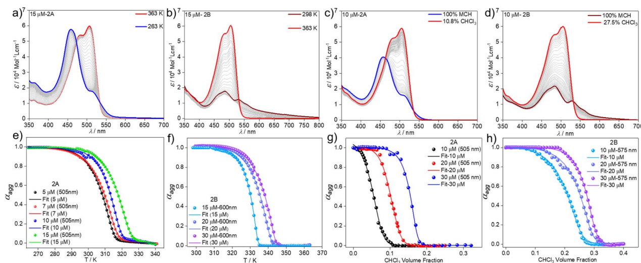
Fig. 3 VT UV-vis studies in MCH ( c = 1.5 \times 10^{-5} \text{ M} ) with a cooling/heating rate of 1 \text{ K min}^{-1} for 2\mathbf{A} (a) and 2\mathbf{B} (b). Plot of \alpha_{\text{agg}} vs. temperature monitored at \lambda = 505 \text{ nm} for 2\mathbf{A} (e) and at \lambda = 600 \text{ nm} for 2\mathbf{B} (f) and corresponding fits to the nucleation–elongation model. UV-vis studies at different MCH– \text{CHCl}_3 ratios ( c = 1 \times 10^{-5} \text{ M} ) and 298 \text{ K} for 2\mathbf{A} (c) and 2\mathbf{B} (d). Plot of \alpha_{\text{agg}} vs. \text{CHCl}_3 volume fraction along with corresponding fits to the nucleation–elongation model for 2\mathbf{A} ( \lambda = 505 \text{ nm} ) (g) and 2\mathbf{B} ( \lambda = 575 \text{ nm} ) (h).
