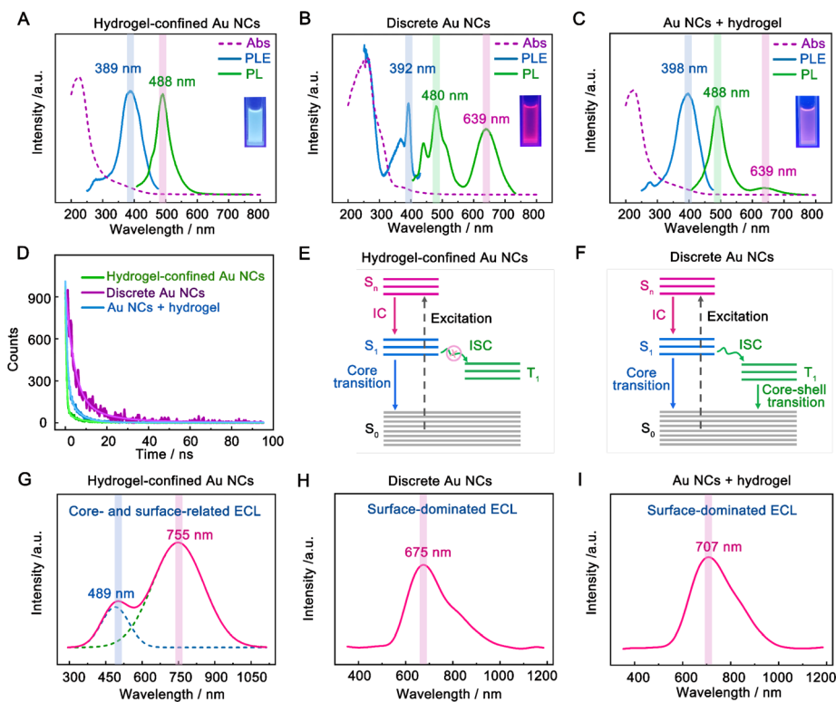
Fig. 2 Optical characterization of hydrogel-confined Au NCs. UV-vis absorption (purple line), PLE (blue line), and PL (green line) spectra of (A) hydrogel-confined Au NCs, (B) discrete Au NCs, and (C) the mixture of Au NCs and the hydrogel. (D) PL decay profiles of hydrogel-confined Au NCs, discrete Au NCs, and the mixture of Au NCs and the hydrogel. Schematic diagram of the excited state relaxation dynamics of (E) hydrogel-confined Au NCs and (F) discrete Au NCs. S_0 ground state, S_1 lowest singlet state, S_n high singlet state, T_1 lowest triplet state, IC internal conversion, and ISC intersystem crossing. ECL spectra of (G) hydrogel-confined Au NCs, (H) discrete Au NCs and (I) the mixture of Au NCs and the hydrogel obtained by scanning from 0 to 1.5 V in 0.1 M PBS (pH 7.4) solution with 50 mM TEA as the co-reactant.
