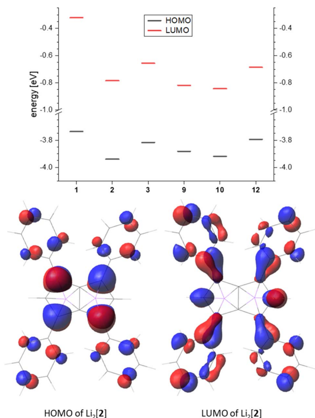
Fig. 7 Top: frontier orbital energy levels of the calculated pentalenides in eV (B3LYP/6-311+G*, PCM(THF)). Bottom: representative frontier orbitals (isovalue 0.035).
