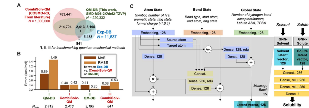
Fig. 1 (A) The three databases for evaluating theoretical methods against experimental solubilities. (B) Accuracy comparisons of CombiSolv-QM and QM-DB for the data points overlapping with Exp-DB . (C) Architecture of the graph neural network for solubility. ASA: accessible surface area, TPSA: topological polar surface area.
