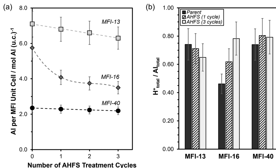
Fig. 2 (a) Total Al content per MFI unit cell (96 T atoms) and (b) bulk H + tot /Al tot molar ratio as a function of the number of AHFS-treatment cycles. Dashed lines in (a) serve to guide the eye. Error bars in (a) reflect uncertainties ( \pm 10\% in (a) and \pm 15\% in (b)).
