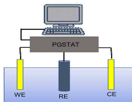
Fig. 2 Illustration for the three-electrode setup used in the photoelectrochemical technique. WE = working electrode (Sb 2 S 3 thin films); RE = reference electrode (SCE); CE = counter electrode (Pt plate).
