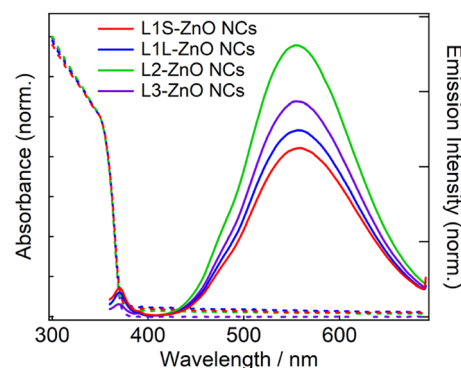
Fig. 3 Steady-state absorption and emission spectra of ZnO NCs in chloroform capped with different phosphonic acids at room temperature. The excitation wavelength is 350 nm.
