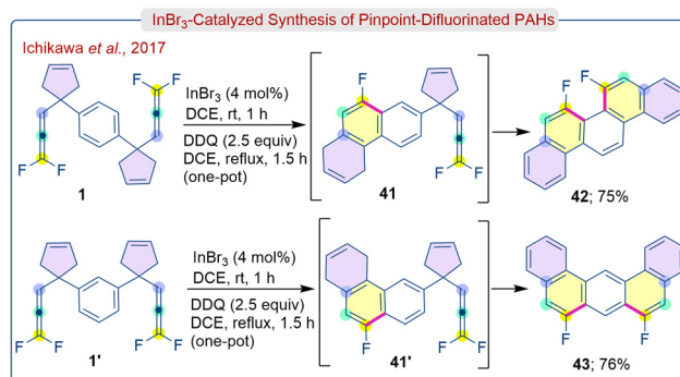
Scheme 22 In(III)-catalyzed synthesis of F 2 -PAHs from bis(1,1-difluoroallenyl) compounds.
