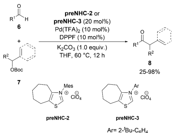
Scheme 4 NHC/Pd synergistically catalysed \text{C}(\text{sp}^2)\text{-H} benzylation or allylation of general aldehydes.
