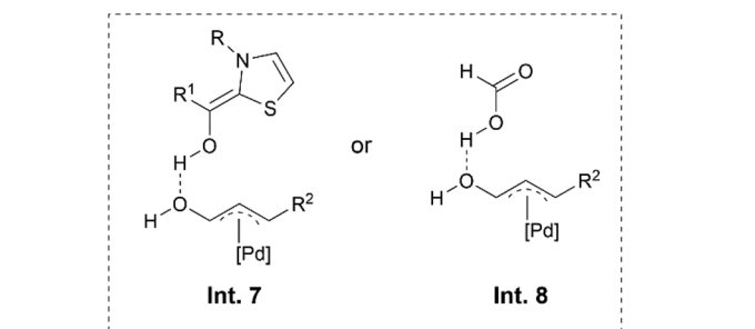
Scheme 6 Synthesis of \beta,\gamma -unsaturated ketones by NHC/Pd synergistic catalysis.
