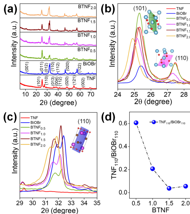
Fig. 1 (a) XRD diffraction patterns of pristine \text{TiO}_2 nanofiber (TNF); BiOBr; and heterojunctions of \text{BTNF}_{0.5} , \text{BTNF}_{1.0} , \text{BTNF}_{1.5} , and \text{BTNF}_{2.0} . (b and c) Magnified portion of the spectra from 23\text{--}28^\circ of TNF and 29\text{--}35^\circ of BiOBr with an inset crystal structure with (101) and (110) planes, respectively, and (d) effect of the intensity ratio of \text{TNF}_{110}/\text{BiOBr}_{110} with an increase in BiOBr content.
