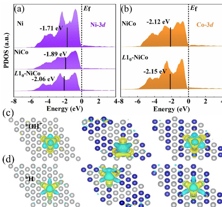
Fig. 2 (a) The density of states and d-band center of Ni and (b) Co atoms, (c) the differential charge density diagram of \text{*OH}^- and (d) \text{*H} of Ni, disordered NiCo solid solution and ordered intermetallic L_{10} -NiCo.
