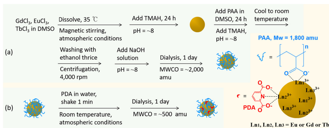
Fig. 1 Syntheses of (a) \text{GdEu}_x\text{Tb}_{1-x}\text{O}_3@(\text{PAA}) nanoparticles and (b) \text{GdEu}_x\text{Tb}_{1-x}\text{O}_3@(\text{PAA}/\text{PDA}) nanoparticles ( x = 0, 0.1, 0.3, 0.5, 0.7, 0.9 , and 1 ).
