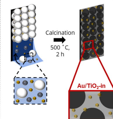
Fig. 1 Schematic illustration of Au/TiO 2 IO film synthesis in which Au NPs are placed either (a) on the TiO 2 surface via a two-component co-assembly approach, or (b) in the TiO 2 matrix via a three-component co-assembly approach.
