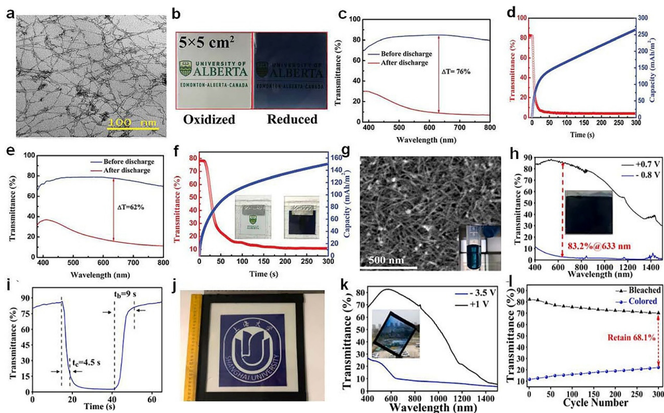
Fig. 9 (a) TEM image of the MTWO. (b) Photographs, (c) transmittance spectra, and (d) self-coloring (discharge) process of a MTWO cathode. (e) Transmittance spectra, (f) self-coloring process of the Zn-based EC device. (a–f) Adapted with permission from ref. 72. Copyright 2019, Wiley-VCH. (g) SEM image, (h) transmittance spectra, (i) switching speed of \text{W}_{17}\text{O}_{47}/\text{NaWO}_3 NW electrode. (j) Photograph, (k) transmittance spectra, and (l) cycling stability of the prototype MED. (g–l) Adapted with permission from ref. 73. Copyright 2021, Elsevier.
