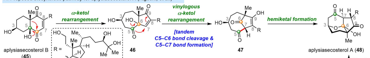
A. Proposed biosynthetic pathway for aplysiasecosterol A (Kigoshi, et al.)
