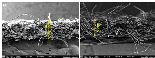
Fig. 10 FESEM images of (A) coated and (B) uncoated fabric.
