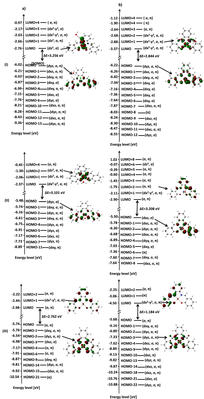
Fig. 13 Frontier molecular orbital energy level diagram: (a) in the ground state and (b) in the excited state, low spin. (I) [Fe(SALPHEN)Cl(H 2 O)]; (II) [Co(SALPHEN)(H 2 O)]; and (III) [Cu(SALPHEN)].
