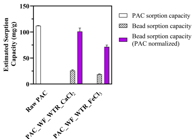
Fig. 7 Imidacloprid sorption capacities of raw PAC and BioSorp beads ( n = 3 experimental replicates; error bars represent standard errors of the means. Some error bars are obscured by the data bar plots as the error bars are small). Here, PAC = powdered activated carbon, WF = wood flour, WTR = iron water treatment residuals.
