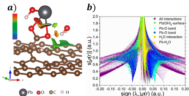
Fig. 6 a) NCI isosurface with s = 0.05 a.u. and b) s[\rho(r)] vs. \text{sign}(\lambda_2)\rho(r) graph for the adsorption Pb(OH)_2 on the GO surface.
