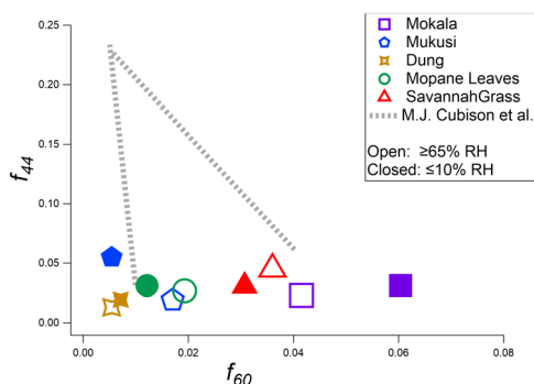
Fig. 3 Primary BBOA composition displayed via f_{60} versus f_{44} from ACSM OA mass spectra of primary BBOA mass under dry ( <10\% RH, closed symbols) or elevated humidity ( \geq 65\% RH, open symbols) conditions in the dark for all fuels used in this work.
