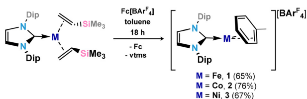
Scheme 1 Synthesis of cationic toluene complexes of Fe ( 1 ), Co ( 2 ), and Ni ( 3 ). Dip = 2,6- \text{tPr}_2\text{-C}_6\text{H}_3 ; \text{Ar}^{\text{F}} = 3,5\text{-(CF}_3)_2\text{-C}_6\text{H}_3 ; Fc = ferrocene.
