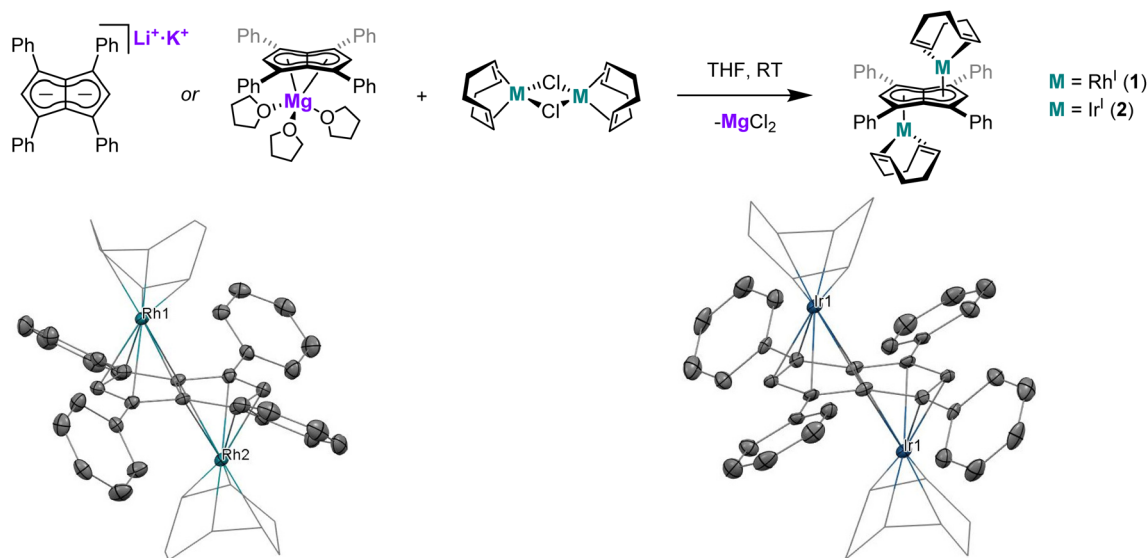
Fig. 1 Synthesis of anti -[Rh I (COD)] 2 [μ:η 5 :η 5 Ph 4 Pn] ( 1 ) and anti -[Ir I (COD)] 2 [μ:η 5 :η 5 Ph 4 Pn] ( 2 ) (top) and corresponding X-ray crystal structures with thermal ellipsoids at the 50% probability level (bottom; hydrogen atoms omitted for clarity).
