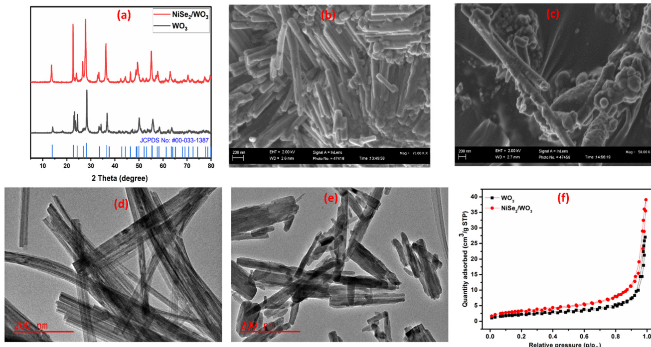
Fig. 1 a) XRD diffraction patterns of \text{WO}_3 and \text{NiSe}_2/\text{WO}_3 , b) SEM image of \text{WO}_3 , c) SEM image of \text{NiSe}_2/\text{WO}_3 , d) TEM image of \text{WO}_3 , e) TEM image of \text{NiSe}_2/\text{WO}_3 , and f) \text{N}_2 sorption isotherms for \text{WO}_3 and \text{NiSe}_2/\text{WO}_3 .
