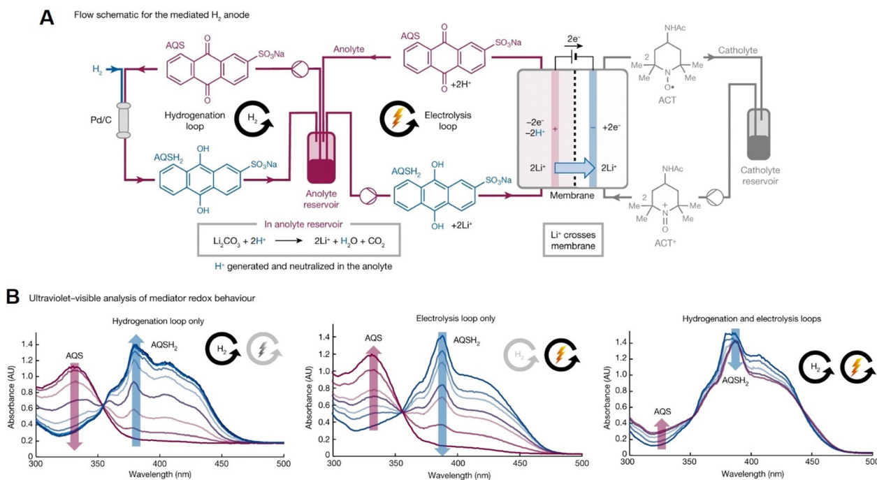
Fig. 18 (A) Schematic of mediated \text{H}_2 anode by pairing the thermal hydrogenation of AQS and the electrochemical oxidation of \text{AQS}\cdot\text{H}_2 in real time. (B) In situ UV-Vis spectra of the redox speciation of AQS and \text{AQS}\cdot\text{H}_2 species in the anolyte reservoir for various processes, such as hydrogenation-only or electrolysis-only loop, or both loops operating simultaneously. Reproduced with permission from ref. 215. Copyright 2023 Springer Nature.
