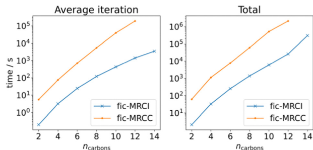
Fig. 3 Polyene calculations at fic-MRCI and fic-MRCC level, using a def2-SVP basis set, while increasing the number of carbons and simultaneously the active space, meaning \text{CAS}(n_{\text{carbons}}, n_{\text{carbons}}) .
