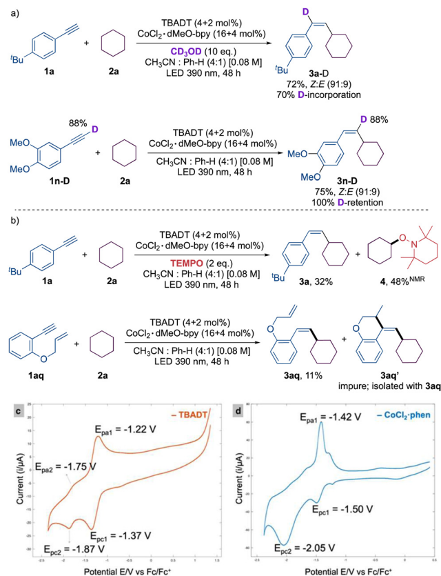
Scheme 2 (a) Deuterium labelling experiments, and (b) radical trap experiments. Cyclic voltammogram of (c) TBADT and (d) \text{CoCl}_2 \cdot 1,10 -phenanthroline.
