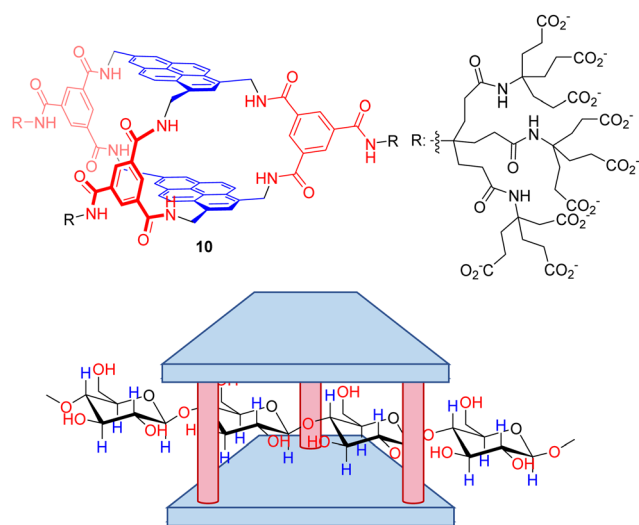
Fig. 9 Macrobicyclic receptor for the binding of \beta -pyranoside polysaccharides in water. The molecular recognition process occurs by threading the biopolymer through the host cavity in a pseudorotaxane structure.
