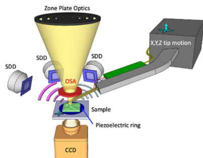
Fig. 1 Combined AFM, XRF and STXM in a single instrument. Sketch of the developed system as deployed at the TwinMic beamline. The monochromatized X-ray beam is incident perpendicularly on the sample plane and is focused through a zone plate diffractive optics while the order sorting aperture (OSA) selects the first diffraction order. The sample is scanned in the X and Y directions on the TwinMic sample stage and the transmitted X-rays are collected using a CCD camera through an X-ray-visible light converting system (not shown here for simplicity). Low-energy X-ray fluorescence (LEXRF) is collected by up to 8 silicon drift detectors (SDDs) in a backscattered configuration. The AFM tip is controlled by an X , Y , Z motor stage.
