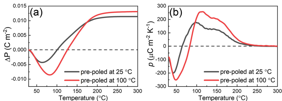
Fig. 6 Temperature-dependent changes in (a) remanent polarization, \Delta P , and (b) pyroelectric coefficient, p , of 0.5 mol% Nb-doped 0.7BF–0.3BT pre-poled at 25 and 100 °C.
