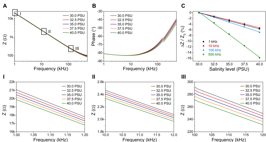
Fig. 3 Electrochemical impedance spectroscopy (EIS) curves of salinity sensors with an exposed sensing area of 500\ \mu\text{m} tested in NaCl solution at salinity levels of 30–40 PSU. (A) Impedance as a function of frequency in the range of 1–500 kHz. Zoom-in EIS curves at frequencies of (I) 1–1.2 kHz, (II) 10–12 kHz, and (III) 100–120 kHz. (B) Phase angle as a function of frequency in the range of 1–500 kHz. (C) Relative impedance change ( \Delta Z/Z_0 , %) as a function of salinity levels at different applied frequencies.
