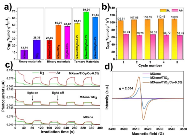
Fig. 12 (a) \text{NH}_4^+ production rate in ambient air; (b) the stability of N 2 photofixation activity of MXene/TiO 2 /Co-0.5% under N 2 and an air atmosphere; (c) photocurrent spectra of MXene, MXene/TiO 2 and MXene/TiO 2 /Co-0.5%; (d) EPR spectra. Reproduced with permission from ref. 163, Copyright 2015 American Chemical Society.
