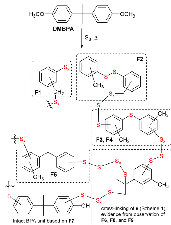
Scheme 2 (A) Microstructures in \text{GS}_{80} (formed by reaction of 80 wt% sulfur with guaiacol). (B) Formation of and microstructures observed in BC90. Substructures are inferred from nine structurally-distinct fragments F1–F9 identified by mass spectrometric analysis of depolymerization products (Chart 1).
