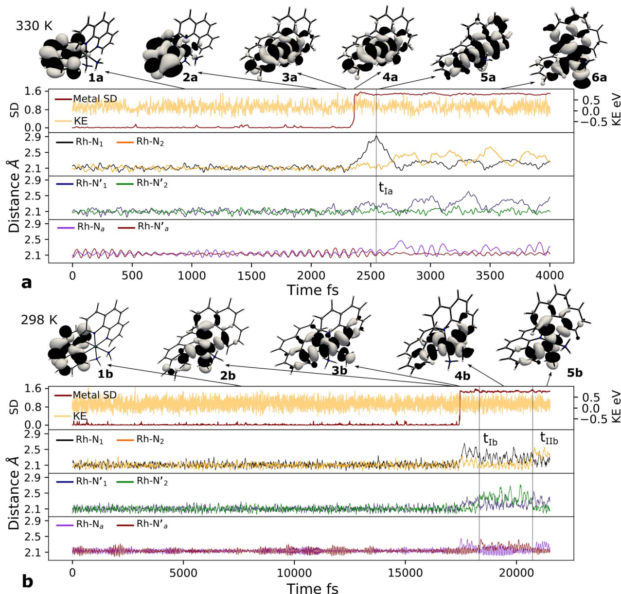
Fig. 4 Metal–ligand bond stretching of [\text{Rh}(\text{III})(\text{phen})_2(\text{NH}_3)_2]^{3+} ( \text{Rh}-\text{N}_1 in black, \text{Rh}-\text{N}_2 in yellow, \text{Rh}-\text{N}'_1 in blue, \text{Rh}-\text{N}'_2 in green, \text{Rh}-\text{N}_a in purple, \text{Rh}-\text{N}'_a in red) before and after ^3\text{LC} \rightarrow ^3\text{MC} crossover reaction, metal spin density (SD) and kinetic energy (KE) fluctuation at temperatures of (a) 330 K, (b) 298 K. ^3\text{SOMO} orbitals are plotted for several snapshots along the simulation.
