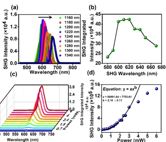
Fig. 8 (a) Wavelength-dependence of the SHG responses in the 1160–1340 nm region, (b) dependence of SHG integrated intensities with varying SHG wavelengths for DPAOCN crystals, (c) power-dependent study of the SHG responses at 610 nm for DPAOCN crystals, and (d) quadratic fit of the SHG intensities with varying excitation power.
