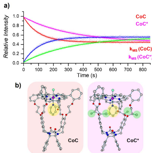
Fig. 6 (a) Relative time evolution of [\text{CoC}(\text{Py})_{\text{IN}}]^+ (red), [\text{CoC}(\text{Py}^{\text{h}})]^+ (blue), [\text{CoC}^*(\text{Py})_{\text{IN}}]^+ (magenta), and [\text{CoC}^*(\text{Py}^{\text{h}})]^+ (green) in a single DRL experiment carried out at 40 °C in \text{CHCl}_3 with 200 equiv. pyridine and 200 equiv. pyridine-D5. Dots are experimental data points, and lines correspond to fittings of experimental data by eqn (S1) and (S2). † (b) DFT-calculated structures of ^1[\text{CoC}(\text{Cl}_{\text{OUT}})(\text{Py}_{\text{IN}})] and ^1[\text{CoC}^*(\text{Cl}_{\text{OUT}})(\text{Py}_{\text{IN}})] optimized with B3LYP-D3/def2svp.
