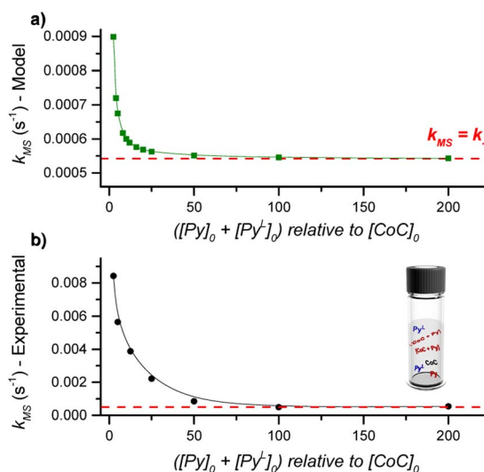
Fig. 3 (a) Evolution of k_{\text{MS}} as predicted by the kinetic model with increasing initial concentrations of (pyridine + pyridine-D5). The rate constants k_1 and k_{-1} were fixed at 50 000 \text{M}^{-1} \text{s}^{-1} and 0.00054 \text{s}^{-1} , respectively. (b) Evolution of k_{\text{MS}} as measured by DRL experiments in \text{CHCl}_3 at 24 °C with increasing equivalents of (pyridine + pyridine-D5). For each experiment, a 1 : 1 ratio of pyridine and pyridine-D5 was used.
