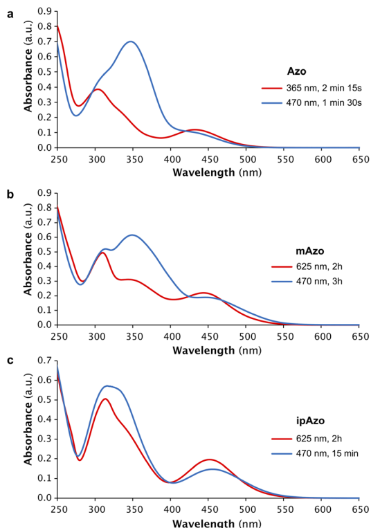
Fig. 2 UV-vis absorption spectra of templates (a) Azo , (b) mAzo , and (c) ipAzo (50 μM in 100 mM sodium phosphate buffer at pH 7.5) showing the photostationary states at the specified wavelengths. The irradiation times required to obtain the different photostationary states are indicated. The spectra showing primarily the cis and trans isomers are depicted in red and blue, respectively.
