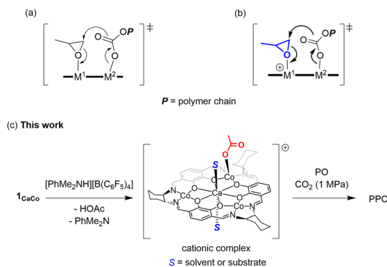
Scheme 1 Key transition state structures of (a) neutral multinuclear catalysts, (b) cationic multinuclear catalysts. (c) This work: alternating copolymerization of PO and \text{CO}_2 by cationic multinuclear species in the presence of anilinium salt.
