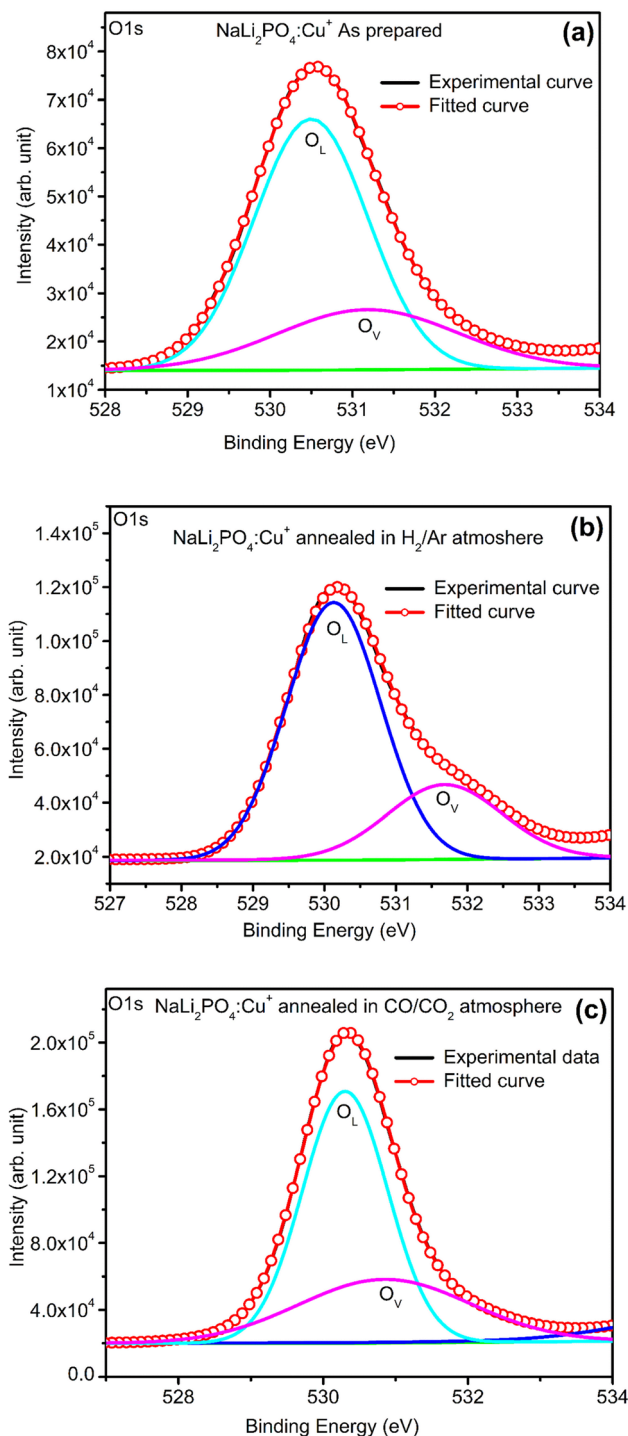
Fig. 10 (a) XPS deconvoluted spectrum of \text{NaLi}_2\text{PO}_4:\text{Cu}(\text{I}) as prepared sample for O 1s and its vacancies, (b) XPS spectrum of \text{NaLi}_2\text{PO}_4:\text{Cu}(\text{I}) annealed in 10% \text{H}_2 in Ar atmosphere at 400 °C for O 1s and its vacancies, (c) XPS spectrum of \text{NaLi}_2\text{PO}_4:\text{Cu}(\text{I}) annealed in \text{CO}/\text{CO}_2 atmosphere at 800 °C for O 1s and its vacancies.
