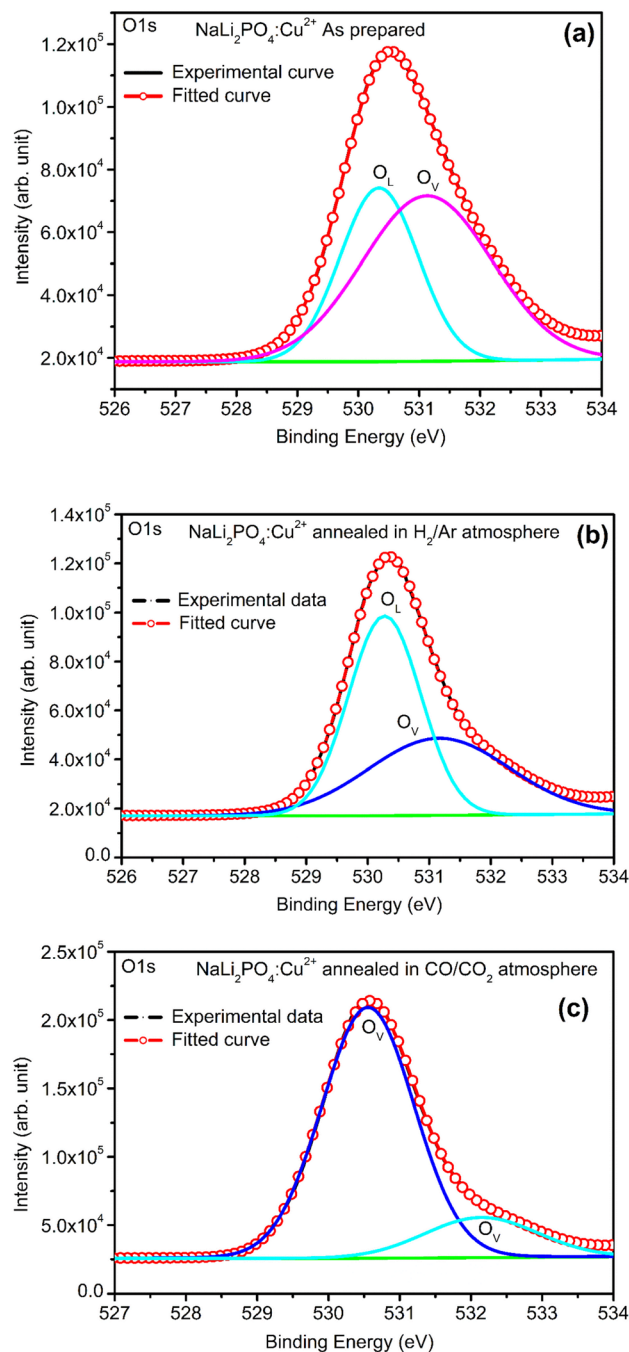
Fig. 11 (a) XPS deconvoluted spectrum of \text{NaLi}_2\text{PO}_4:\text{Cu}(\text{II}) as prepared sample for O 1s and its vacancies, (b) XPS spectrum of \text{NaLi}_2\text{PO}_4:\text{Cu}(\text{II}) annealed in 10% \text{H}_2 in Ar atmosphere at 400 °C for O 1s and its vacancies, (c) XPS spectrum of \text{NaLi}_2\text{PO}_4:\text{Cu}(\text{II}) annealed in \text{CO}/\text{CO}_2 atmosphere at 800 °C for O 1s and its vacancies.
