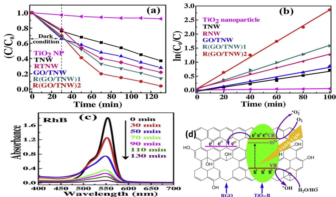
Fig. 9 (a) Plot of (C/C_0) versus time for degradation of RhB in the visible light, (b) kinetics of photodecomposition of the prepared samples, and (c) the absorbance spectra of RhB under visible light irradiation catalyzed by \text{R}(\text{GO}/\text{TNW})_2 composite, and (d) schematic diagram elucidating the mechanism of photocatalytic activity of \text{R}(\text{GO}/\text{TNW})_2 reprinted with permission from ref. 78. Copyright 2022 Elsevier.
