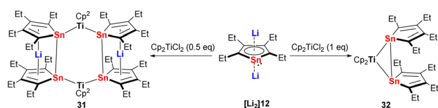
Scheme 5 Reaction of tetraethyldilithiostannole [\text{Li}_2]\textbf{12} with [\text{Cp}_2\text{TiCl}_2] , leading to the formation of 31 and 32 . 33
