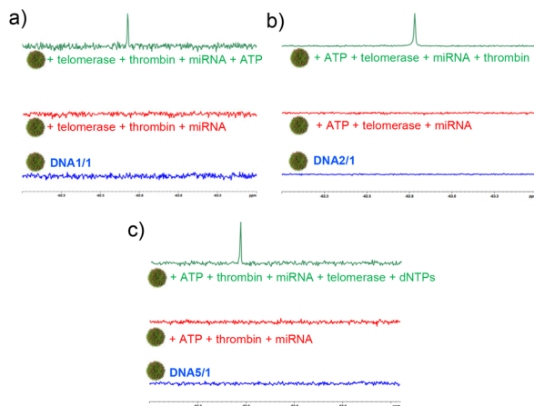
Fig. 4 ^{19}\text{F} -NMR spectral responses of (a) DNA1/1 NPs towards ATP, (b) DNA2/1 NPs towards thrombin and (c) DNA5/1 NPs towards telomerase in the presence of a mixture of other nontargets.
