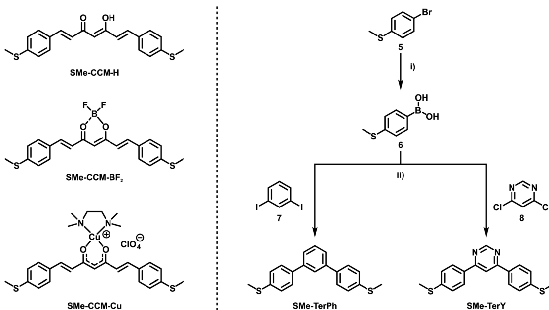
Scheme 4 Previously studied CCM-based congeners with one additional C=C double bond at each side of the ketoenolate chelate and either H, \text{BF}_2 or \text{Cu}^{\text{II}}(\text{tmeda}) as the LA (left). 76 Synthetic route towards reference compounds SMe-TerPh and SMe-TerY (right). (i) (1) n\text{-BuLi} (1.6 M in hexanes), THF, -78^\circ\text{C} , 1 h; (2) \text{B}(\text{O}^i\text{Pr})_3 , -78^\circ\text{C} to rt, 16 h; (3) 1M \text{HCl}_{(\text{aq})} , \text{H}_2\text{O} , rt; (ii) \text{K}_3\text{PO}_4 , \text{Pd}(\text{dppf})\text{Cl}_2 , 1,4-dioxane, 70^\circ\text{C} to 80^\circ\text{C} , 16 h.
