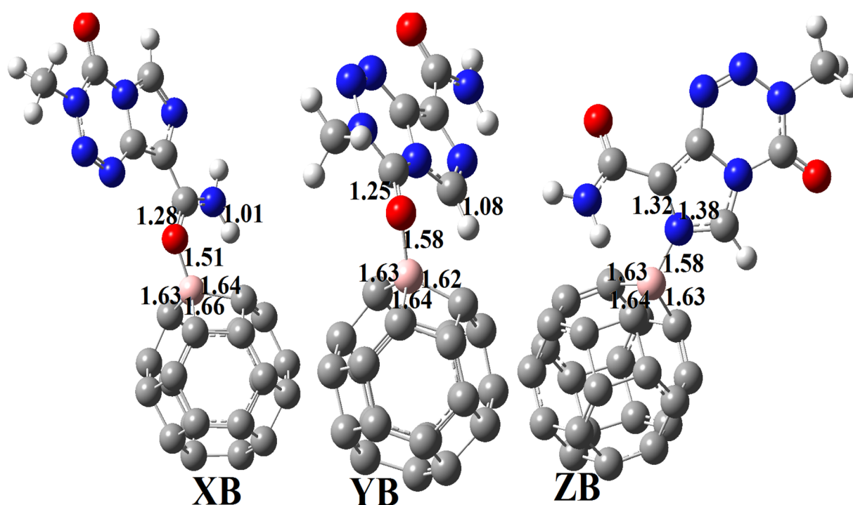
Fig. 4 Optimized structures of XB, YB and ZB obtained at the DFT/M05-2X/6-31+G(d,p) level in the gas phase.
