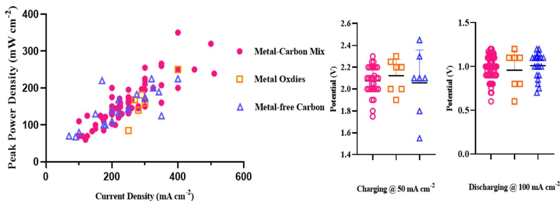
Fig. 23 Performance of different type of catalysts in the zinc-air battery according to reports. 91,100,105,106,128,130,131,133–135,141,144,148,187,189,192,194,198,212,214,216,225,226,240,242,246,248,253–255,257,258,263,267,287,289,290,295,308,314,322,329–385
