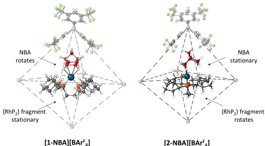
Fig. 10 Packing diagrams contrasting the relative orientations of the NBA and \{\text{RhP}_2\} fragments in [\mathbf{1-NBA}][\text{BAR}^{\text{F}}_4] and [\mathbf{2-NBA}][\text{BAR}^{\text{F}}_4] . The top anion is shown in full along with the B atoms of the other anions within the octahedral array. Carbon atoms of the \sigma -alkane ligands are highlighted in red.
